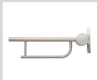
Hinged support rail Stainless steel Support rail in polished stainless steel with hinged support arm 800mm long and concealed fixing plate. L800 x H242 x W110mm Code: S6360MY
